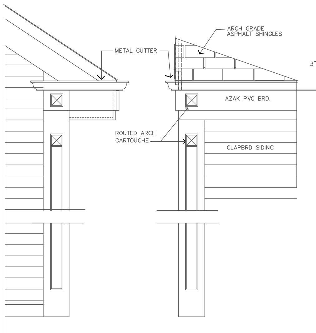
CORNER DETAIL
