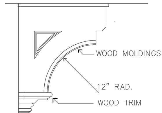
ITALIANATE BRACKET
