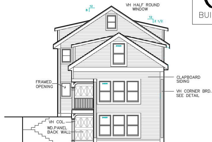
FRONT ELEVATION – (SOUTH)
